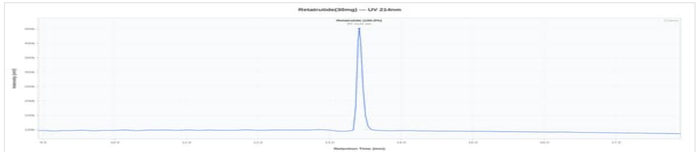
3R-R3 30mg - 3RR330040726J: UV Chromatogram
